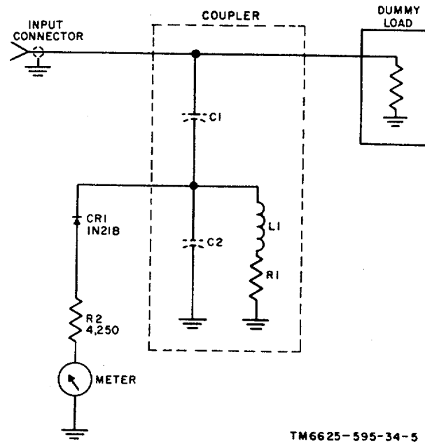
Figure 3-2. Wattmeter ME-8,U, Schematic diagram.
