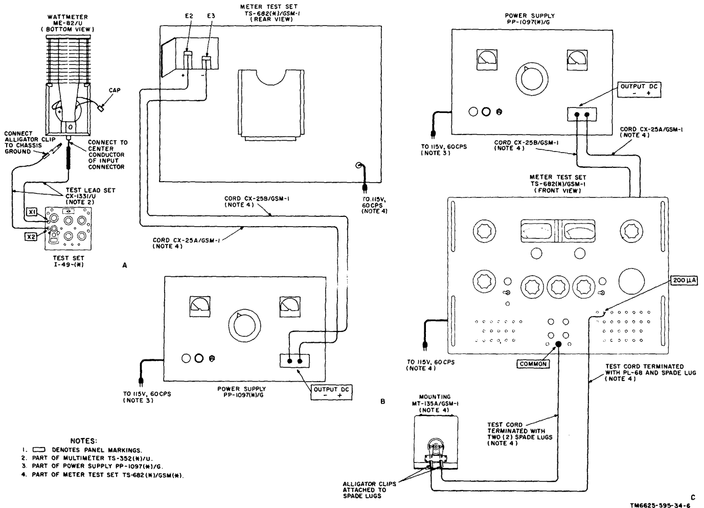
Figure 5-1. General support test setup for crystal, resistance, and meter sensitivity tests.
