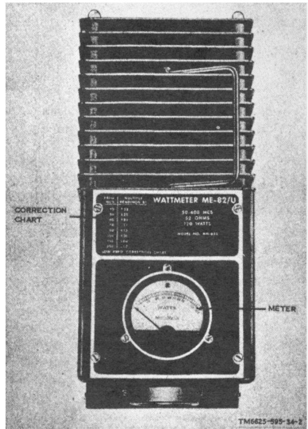
Figure 1-2. Wattmeter ME-82/U, top view.
