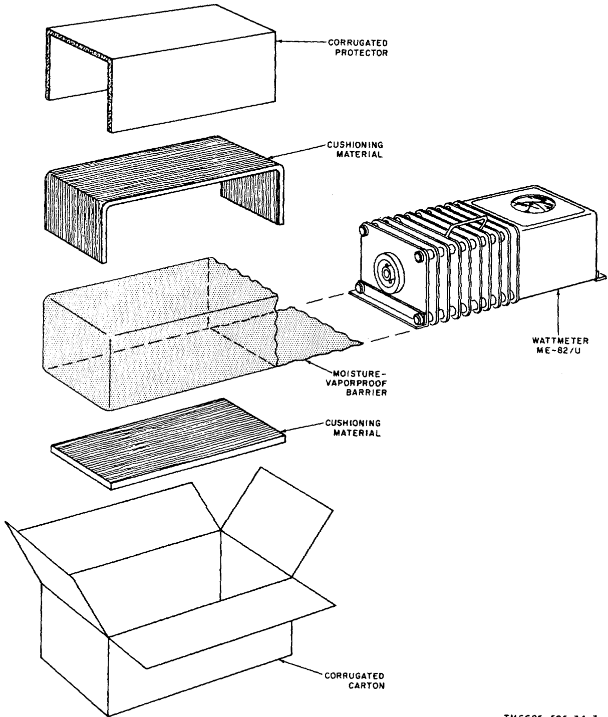
Figure 2-1. Wattmeter ME-821U, packaging diagram.
